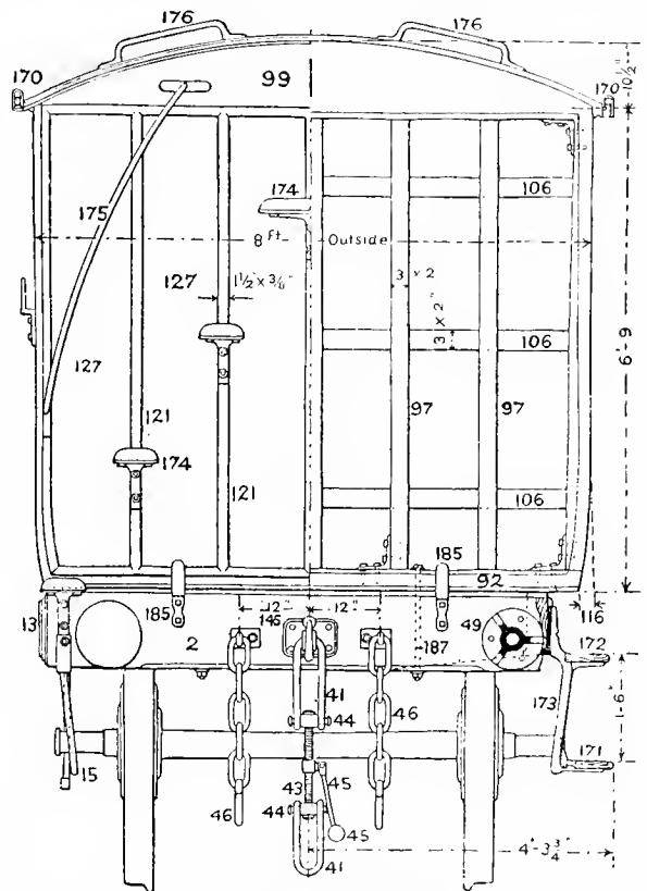
Fig. 504. End Elevation.
